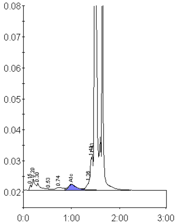
Peak table - ID: 10538325
